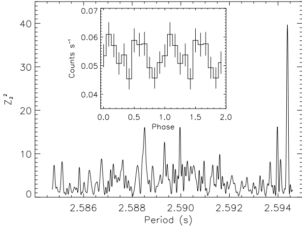
Figure 1. Z_2^2 -periodogram of SGR 1627–41 in the 2–10 keV energy range. The peak at 2.594 39 s is significant at 4\sigma . The inset shows the corresponding pulse profile (2–10 keV, not background-subtracted).
