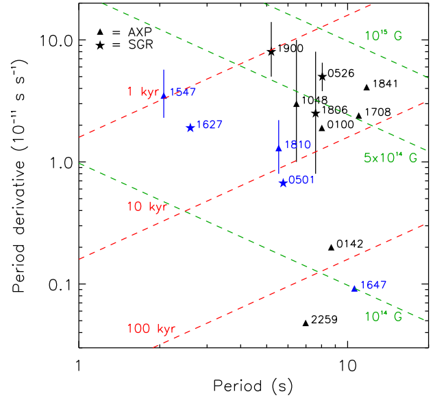
Figure 2. P-\dot{P} diagram for the known magnetars; vertical bars indicate variability ranges. Lines of constant magnetic field strength (green) and characteristic age (red) are indicated. The ‘transient’ magnetars, the ones that show the largest variations of the persistent X-ray flux (up to two or three orders of magnitude), are plotted in blue. Data are from Mereghetti (2008) and our analyses.
